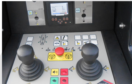
FPC: Full proportional CANbus controls with display
