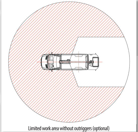
Limited work area without outriggers (optional)
